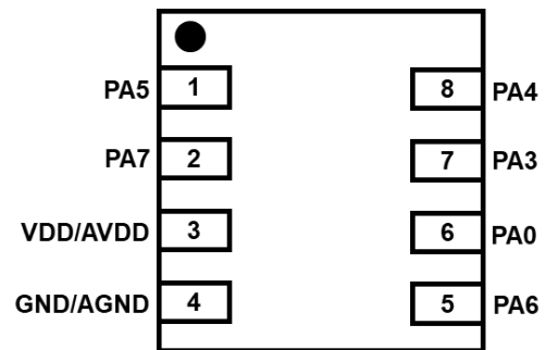
PMS161-2N08B: DFN8 (2*2mm)
