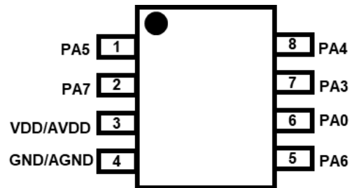
PMS161-S08B: SOP8 (150mil)
